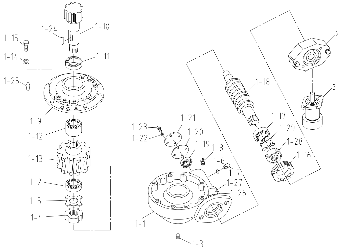
Fig. 3-2 SCS744L SWING R/ G ASS'Y
