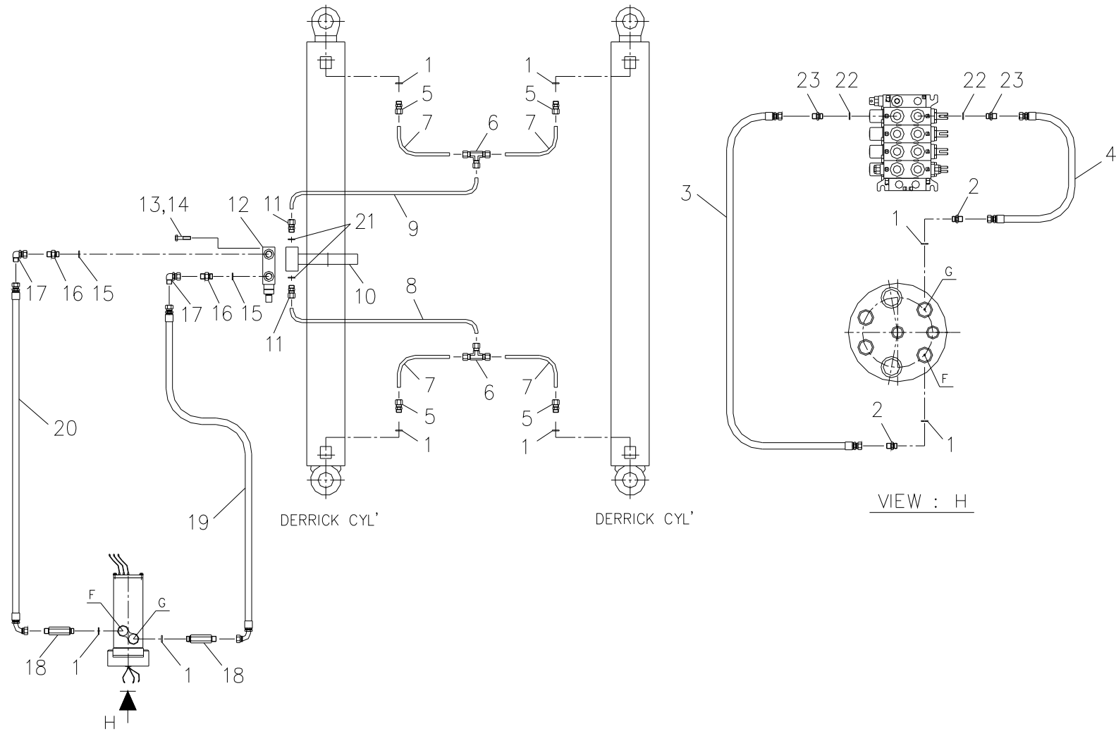
Fig. 5-2 SCS824 DERRICK PIPING
