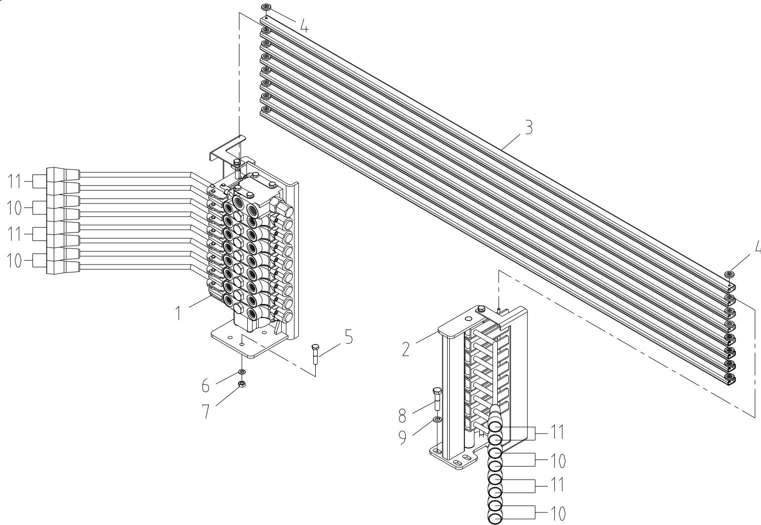
Fig. 3-4 SCS744L OPERATION OUTRIGGER ASS'Y
