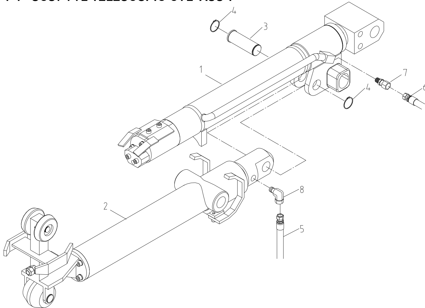
Fig. 1-1 SCS744L TELESCOPIC CYL' ASS'Y
