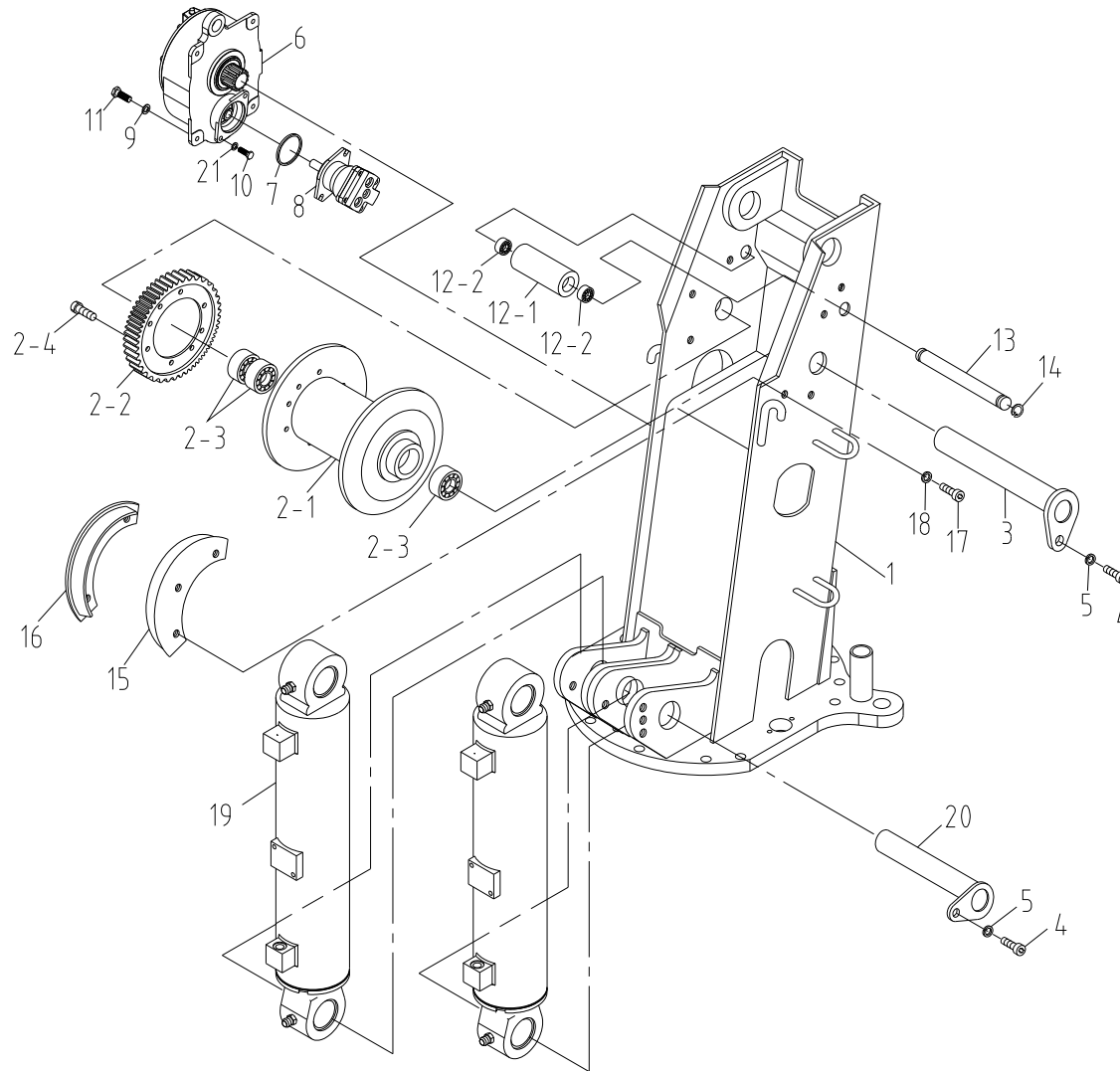
Fig. 2 SCS744L SWING POST ASS'Y
