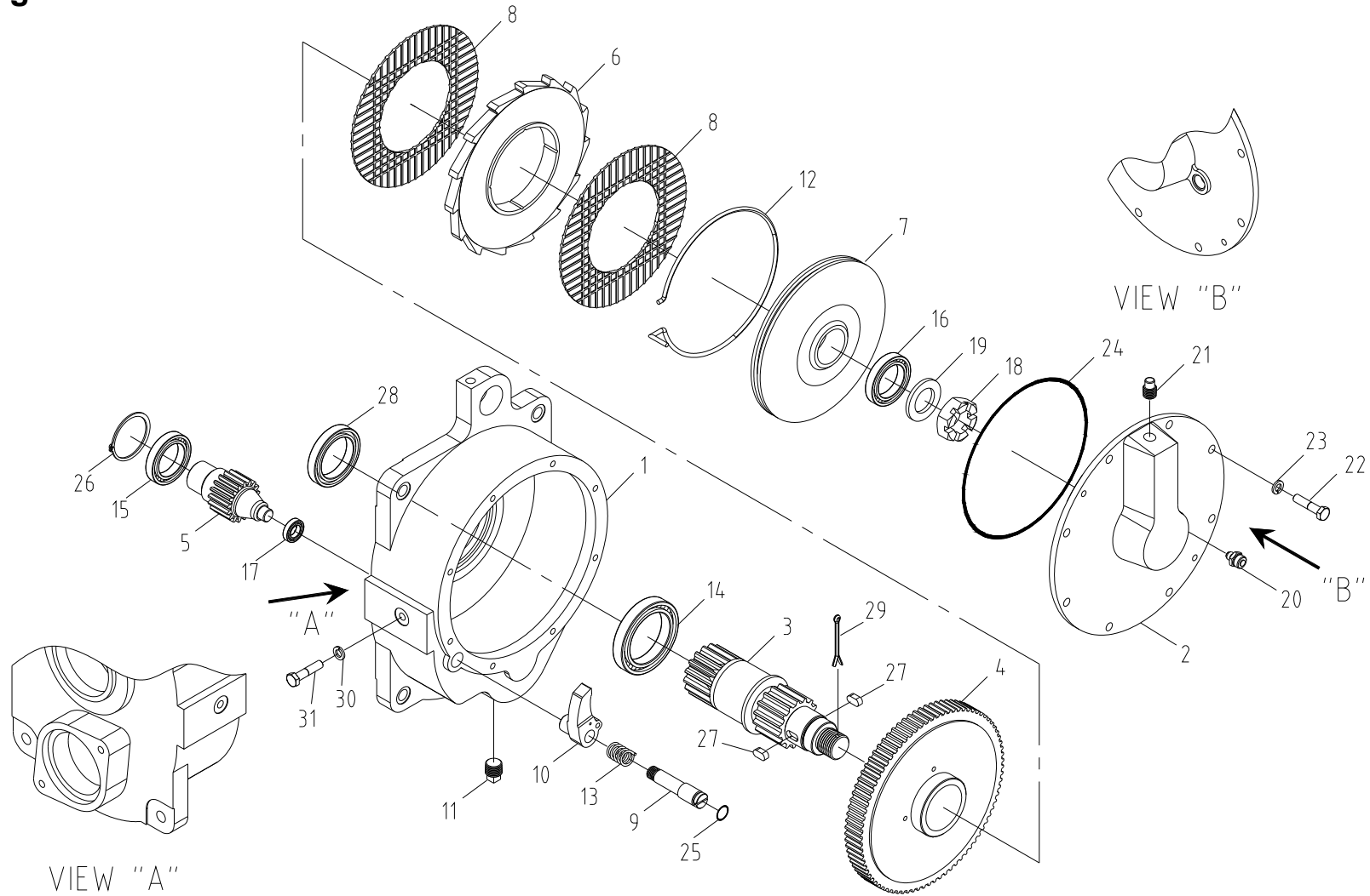
Fig. 2-1 SCS744L WINCH R/ G ASS'Y
