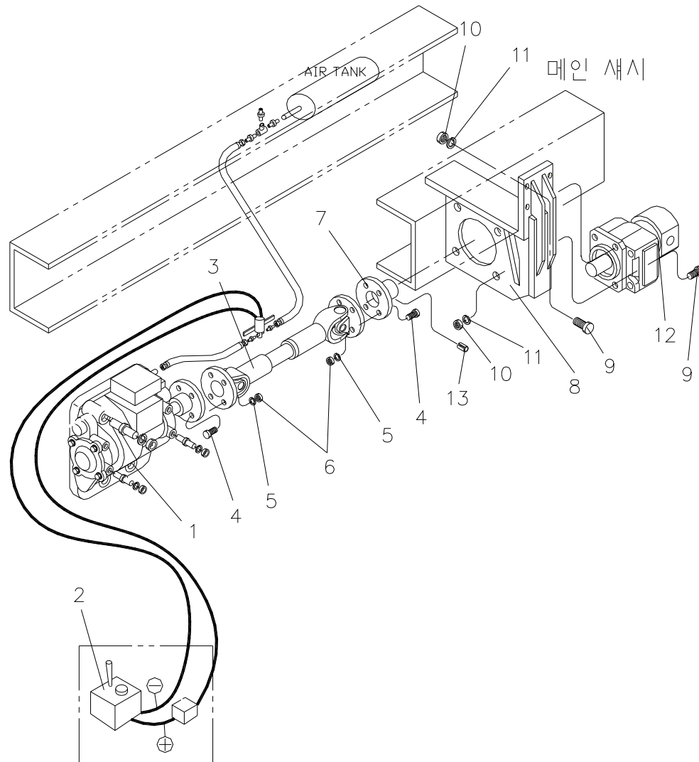
Fig. 8-1 SCS744L P.T.O & PUMP PART(8TON)
