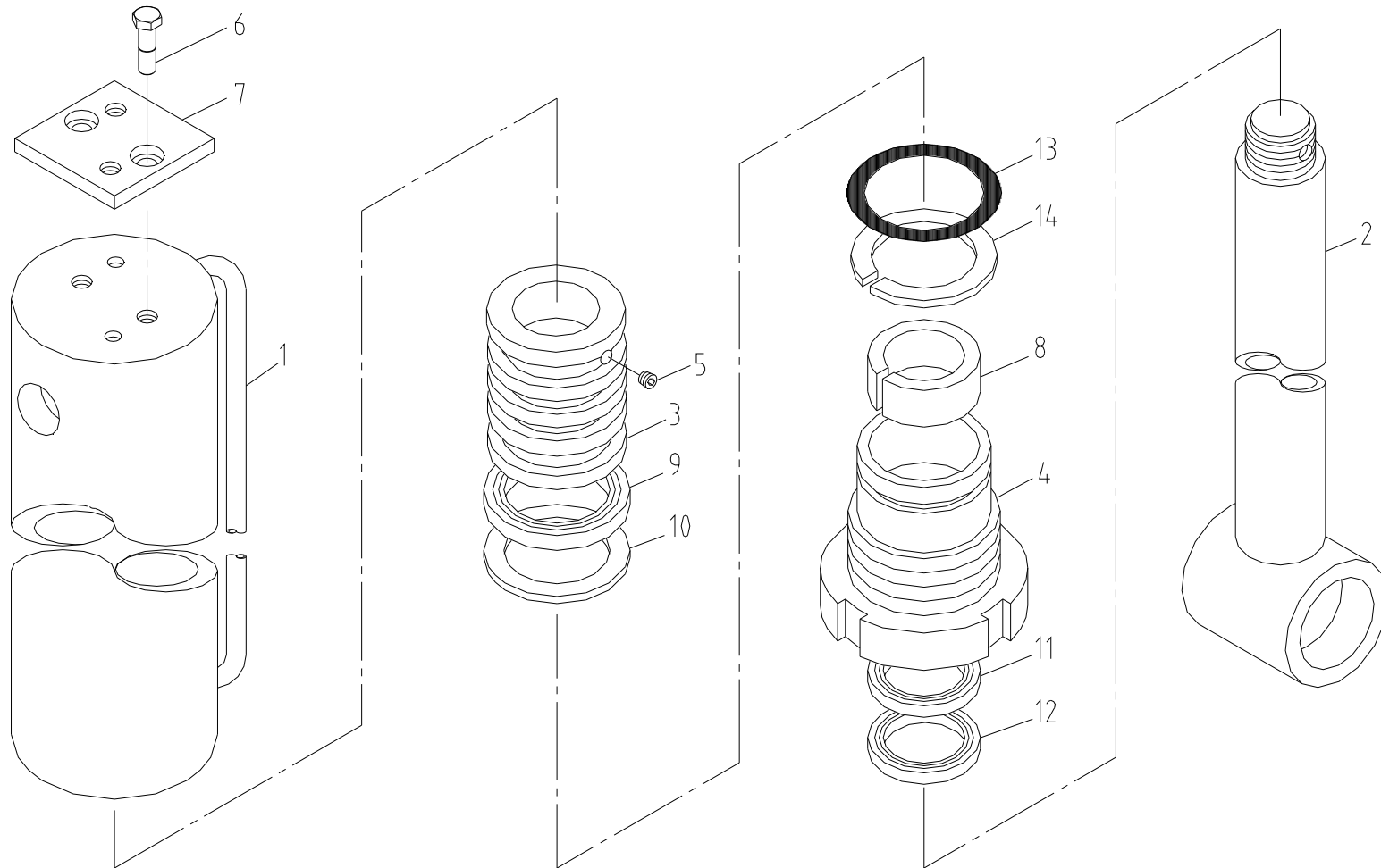
Fig. 4-1 SCS744L JACK CYL' ASS'Y
