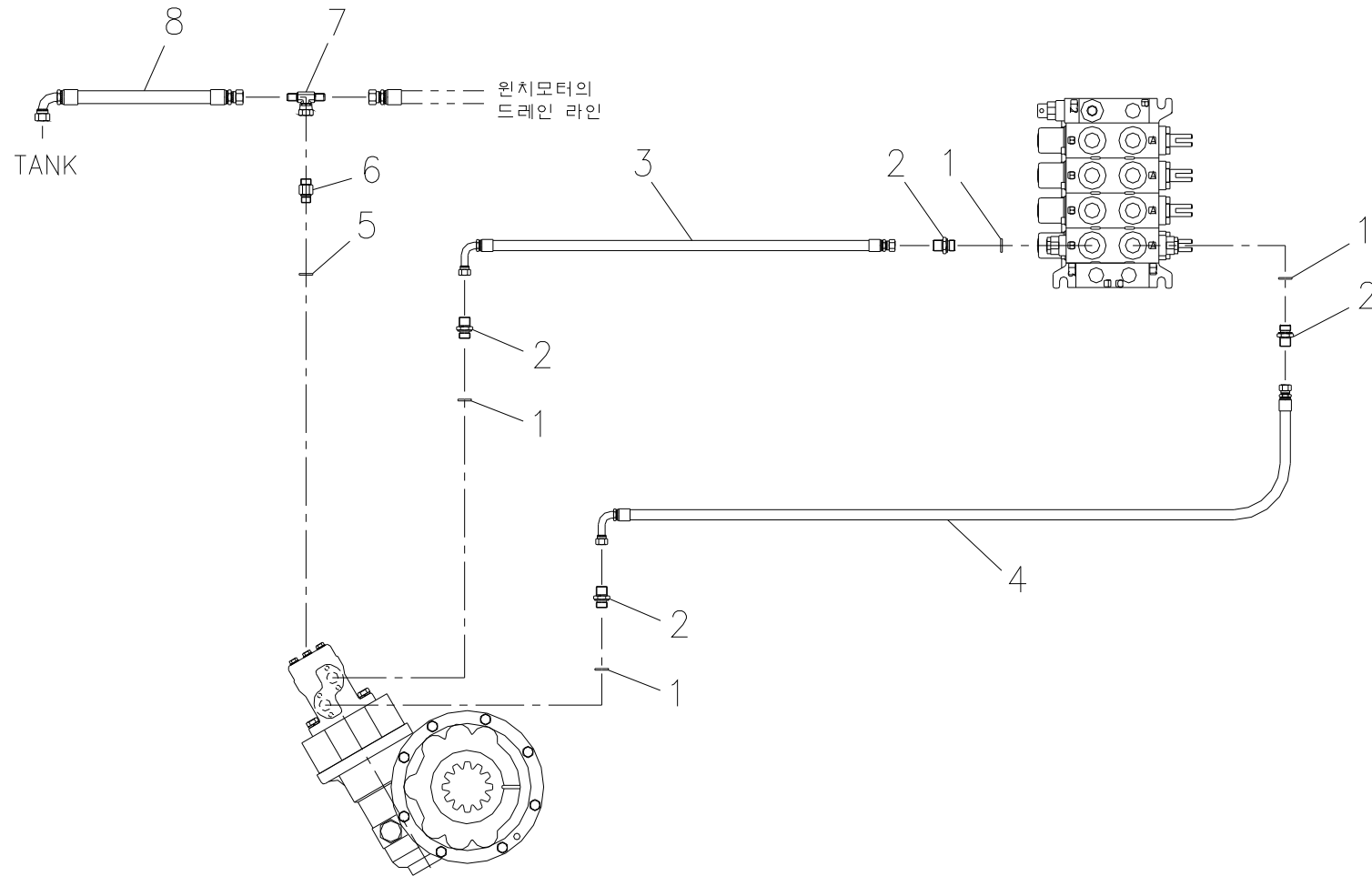
Fig. 5-5 SCS744L SWING PIPING
