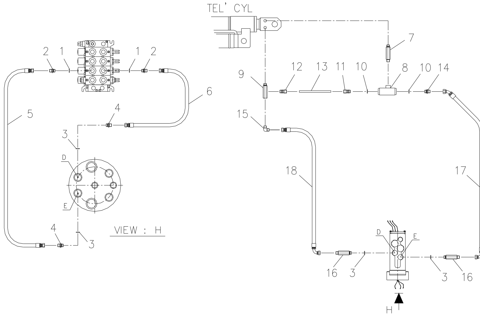
Fig. 5-4 SCS744L TELESCOPIC PIPING
