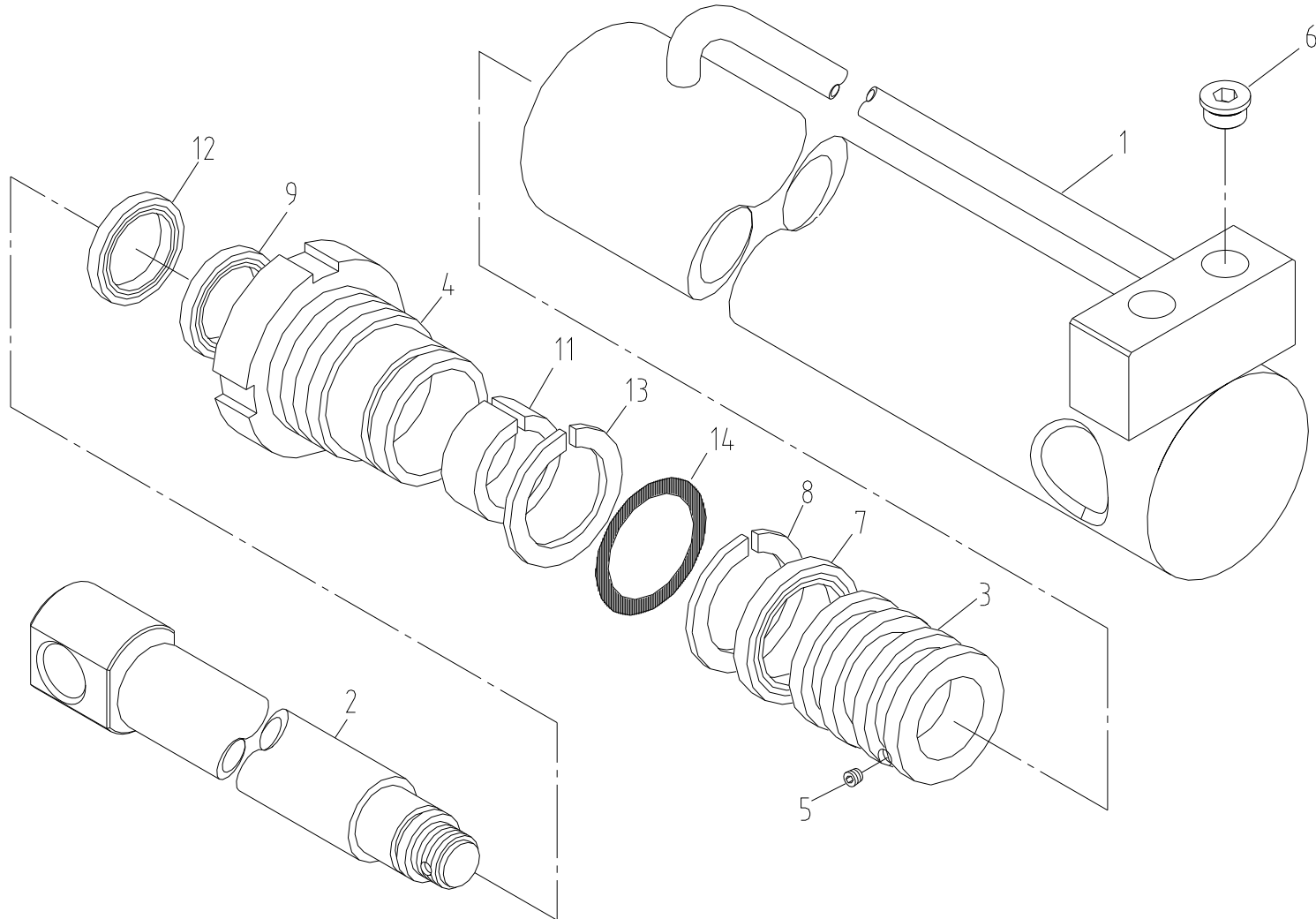
Fig. 4-2 SCS744L EXPANDING CYL' ASS'Y
