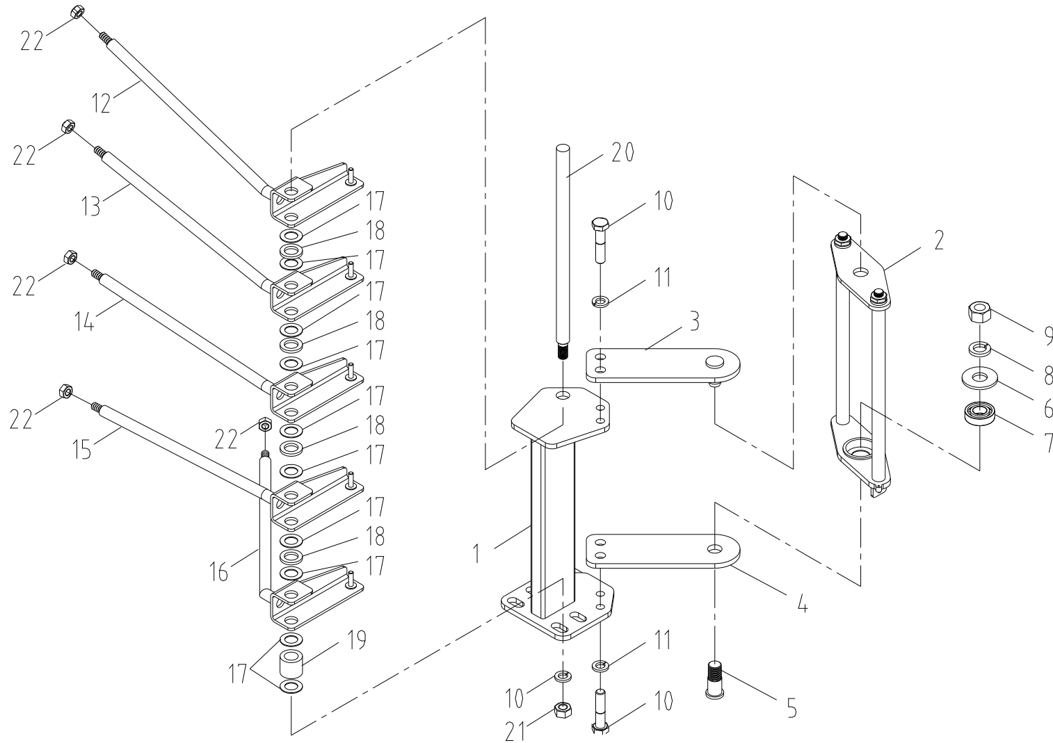
Fig. 3-3-2 SCS744L LEVER STAND SET
