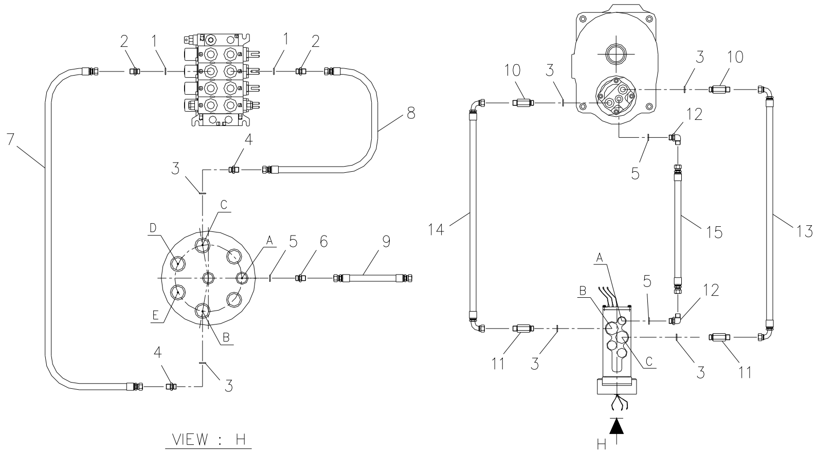
Fig. 5-3 SCS744L WINCH PIPING
