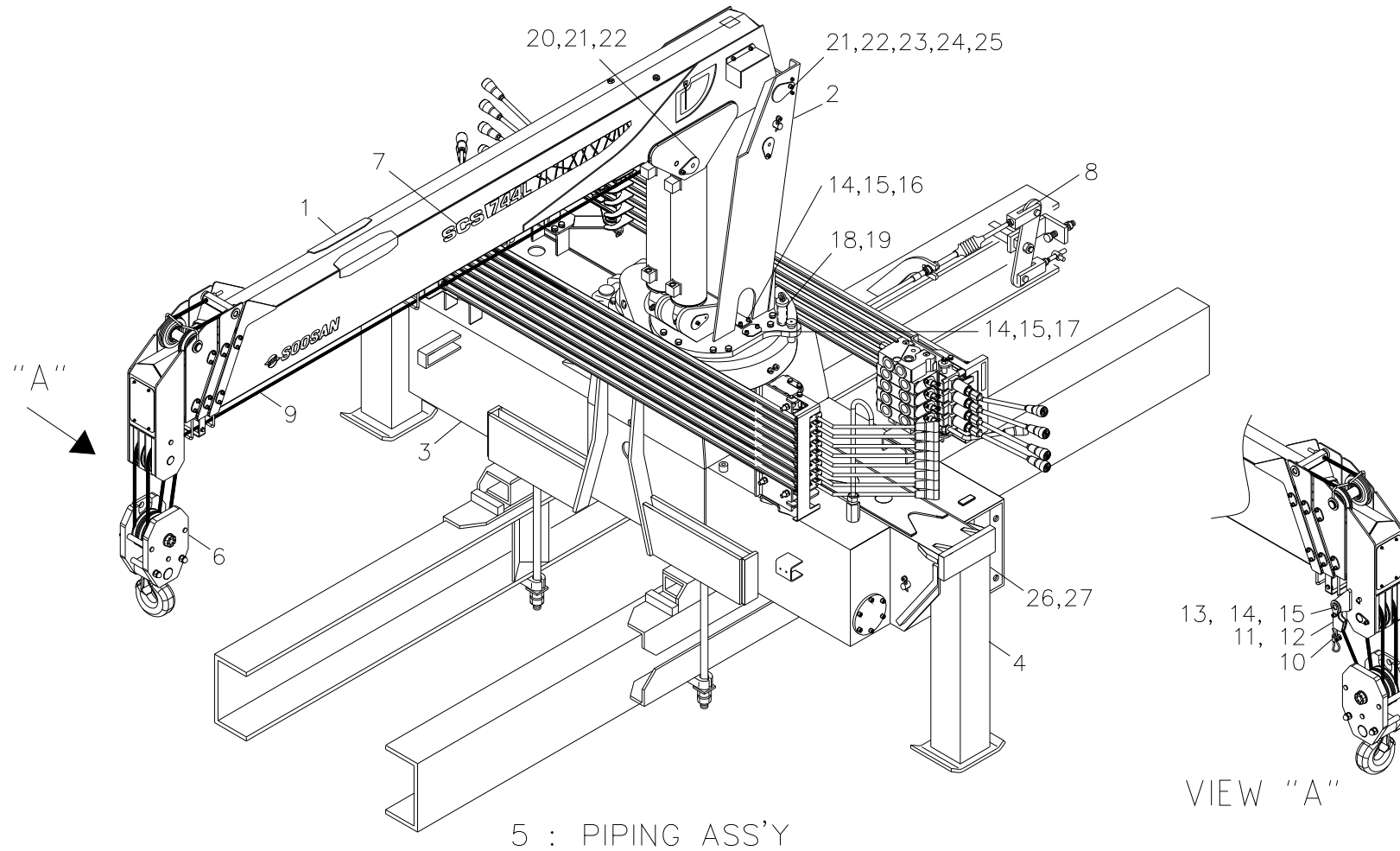
Fig. 0 SCS744L CRANE ASS'Y
