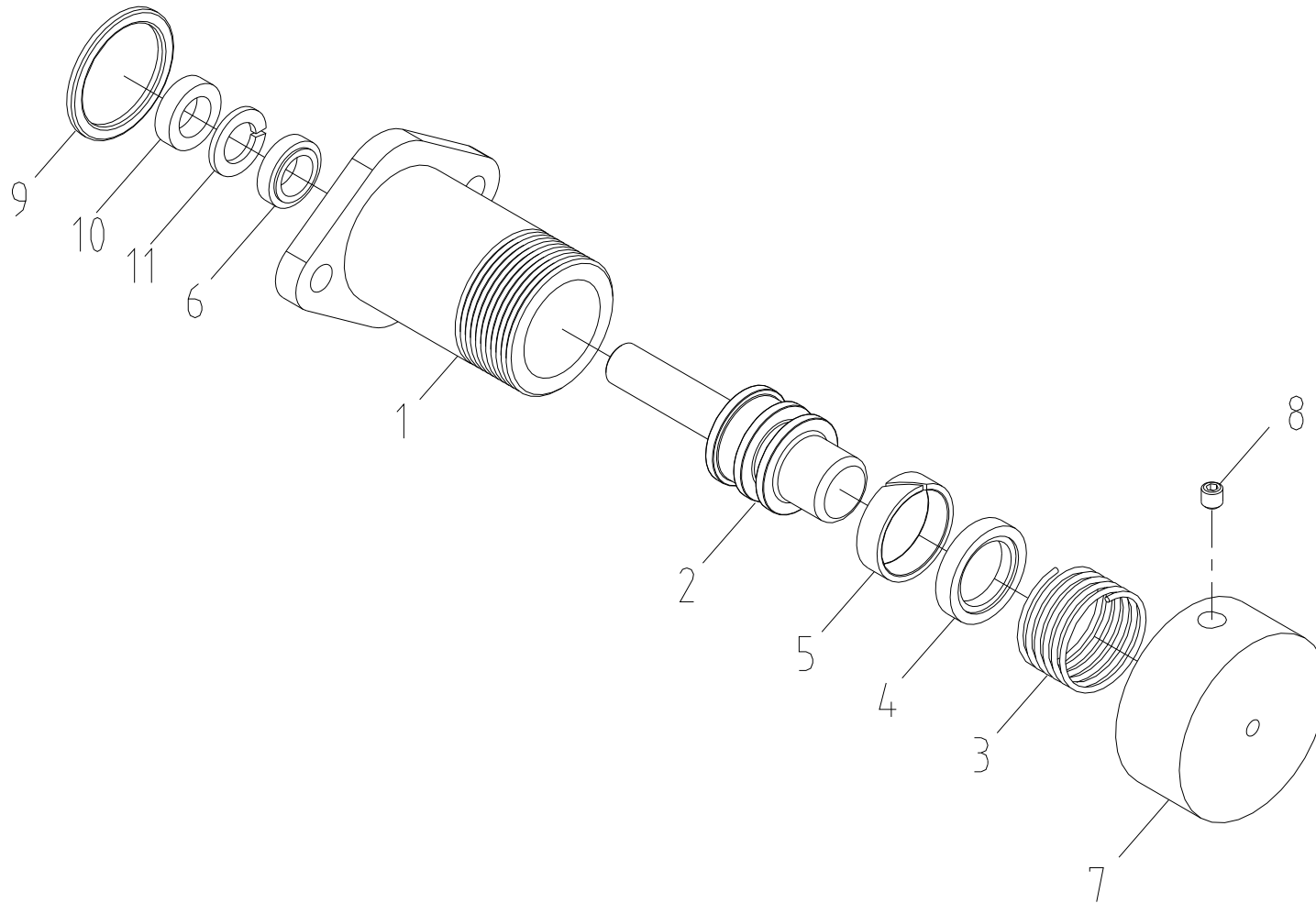
Fig. 3-2-2 SCS744L SWING LOCKING CYL'
