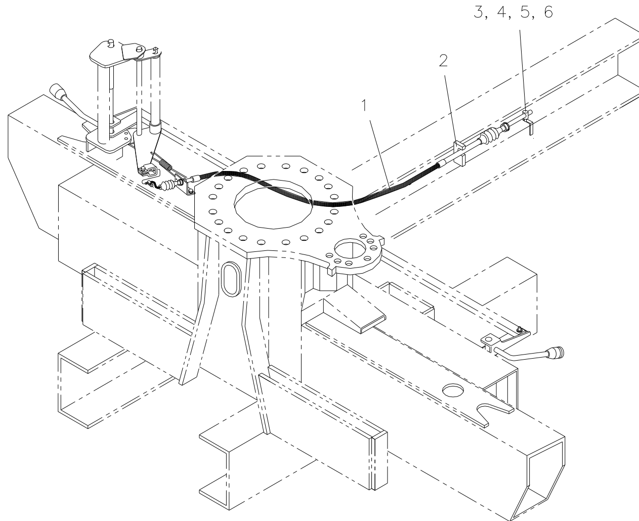
Fig. 8-3 SCS744L ACC'L SYSTEM PART
