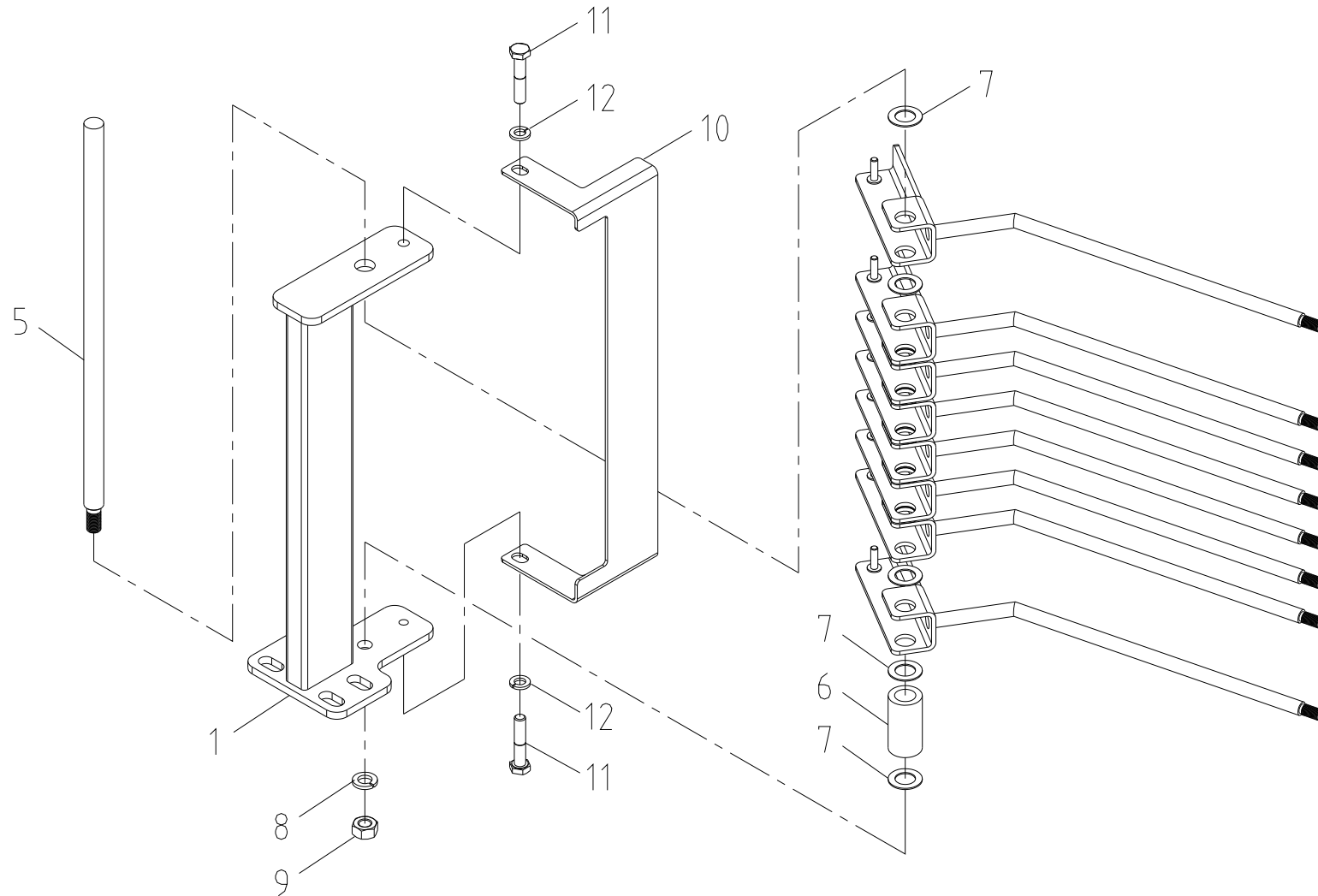
Fig. 3-4-2 SCS744L LEVER STAND SET
