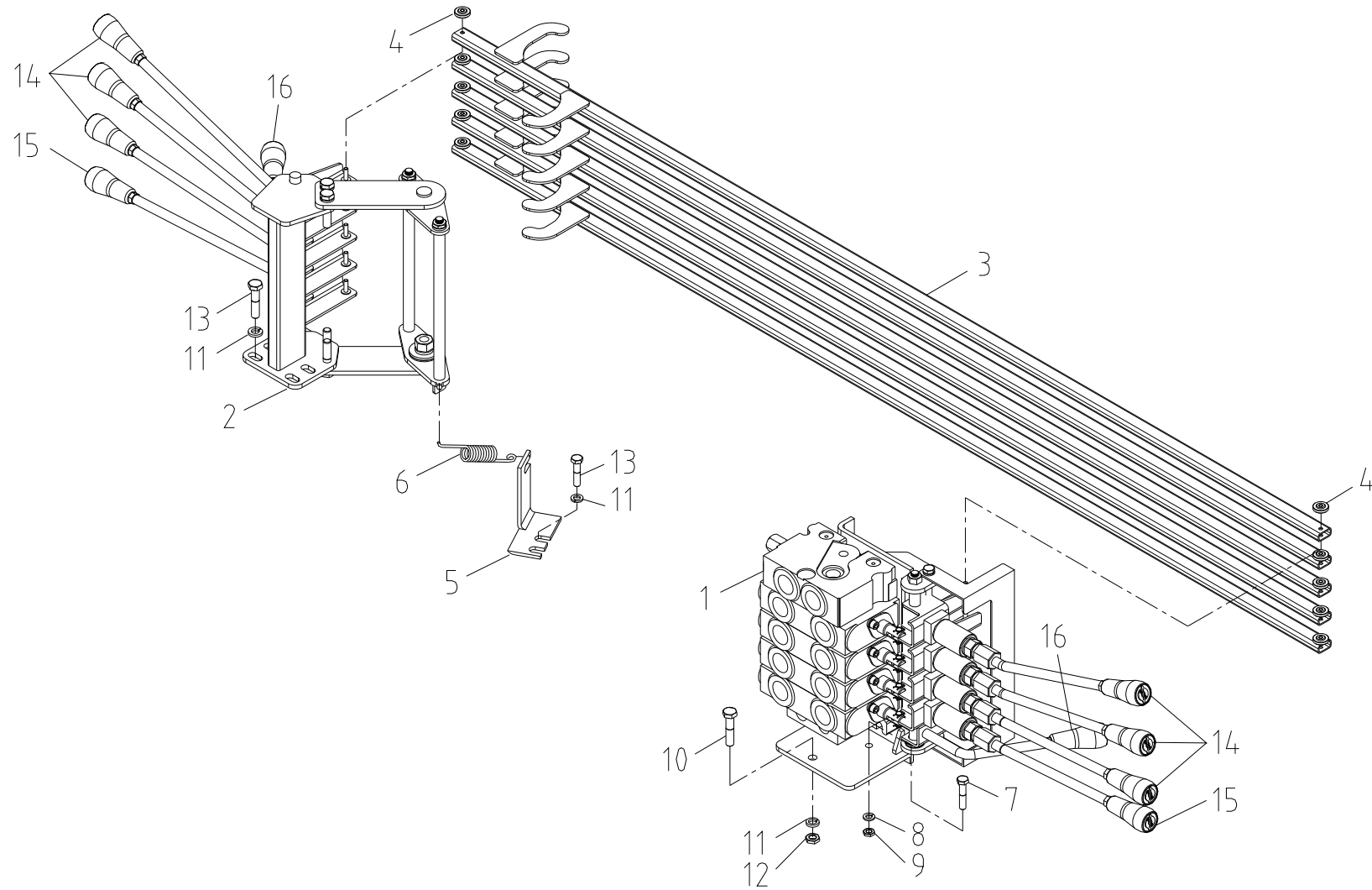
Fig. 3-3 SCS744L OPERATION MAIN ASS'Y
