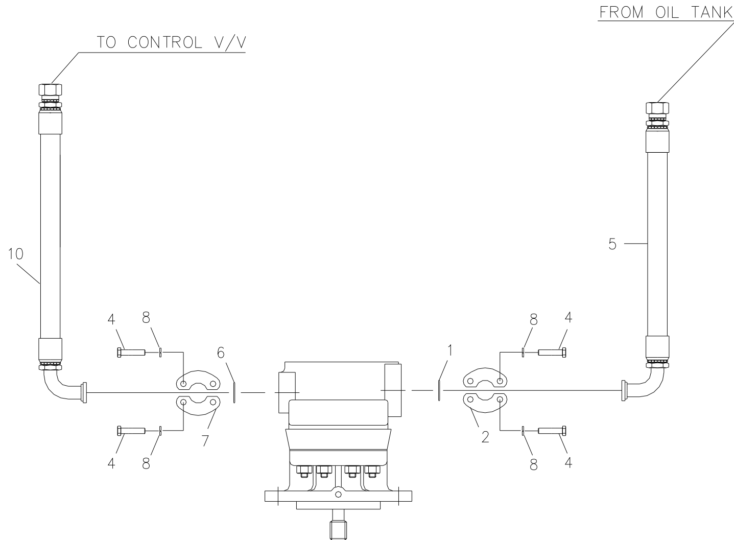
Fig. 8-6 SCS744L M/T PIPING PART
